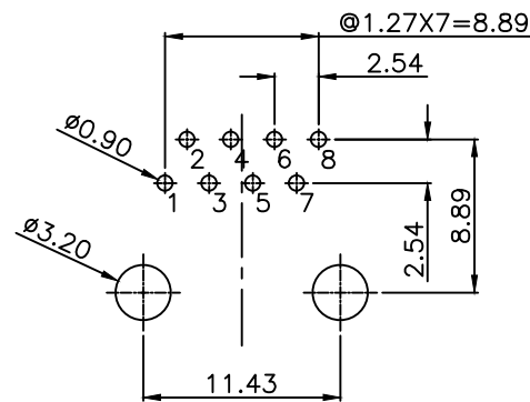
PC Board Layout Component Side Shown PC Board Thickness=1.6mm Tolerance±0.05
